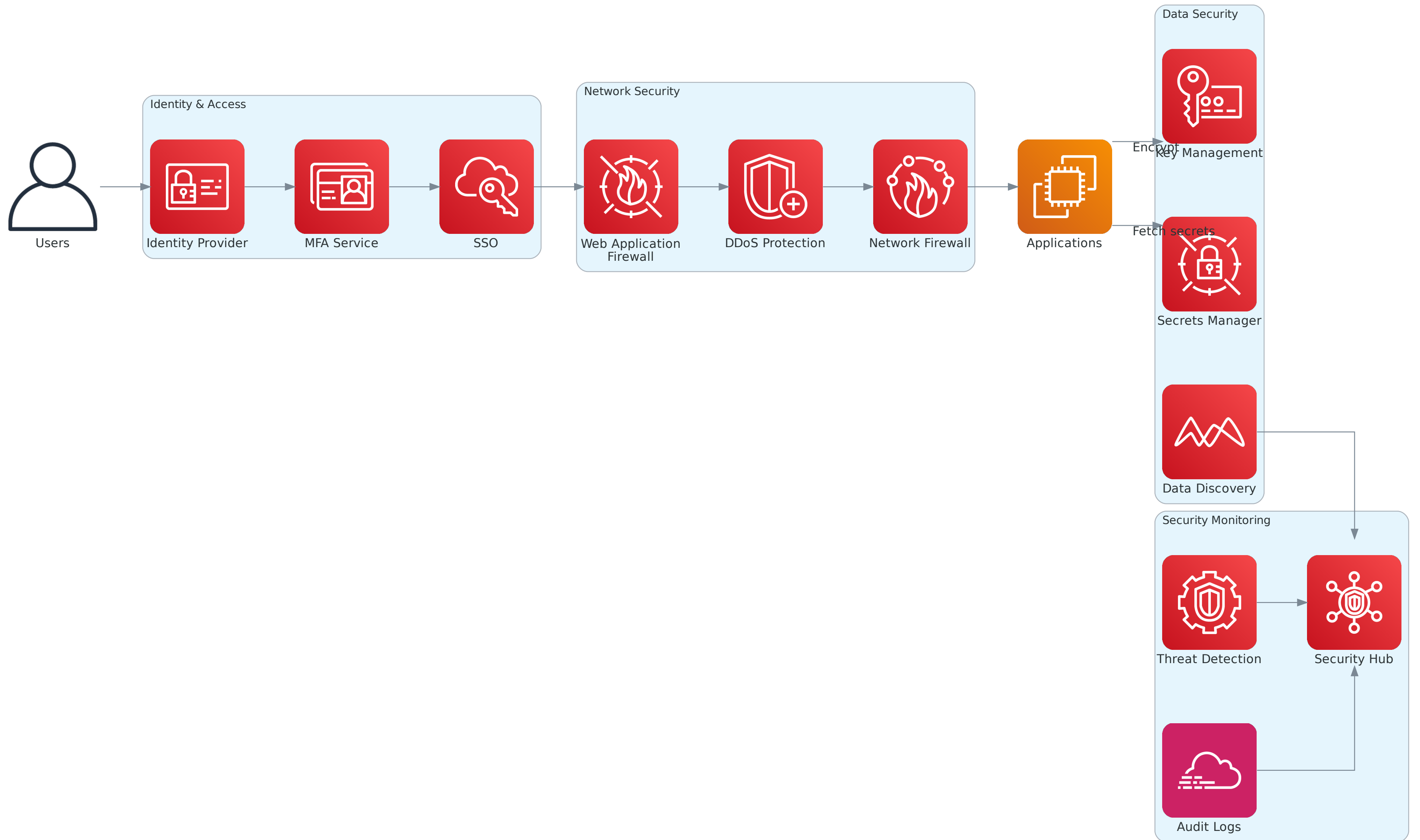
Zero Trust Architecture
